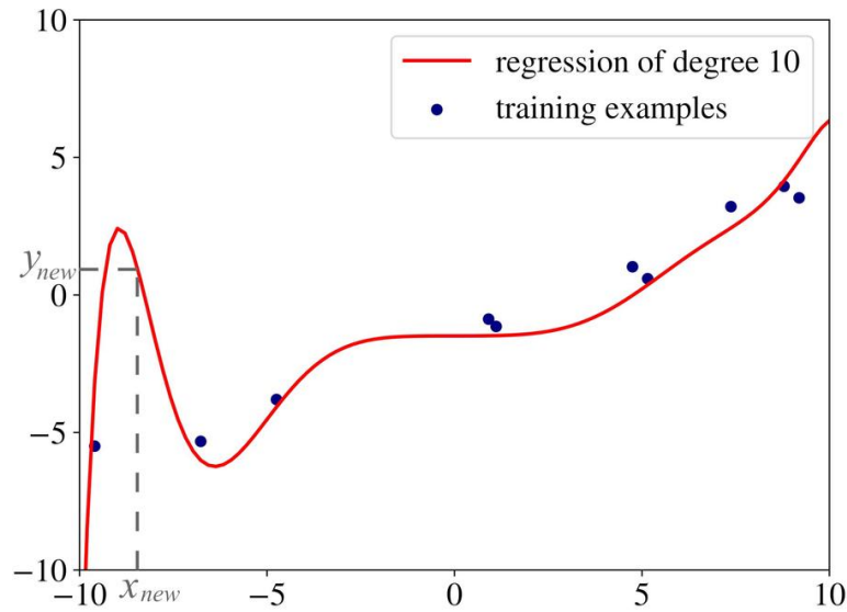
Figure 2: Overfitting.
