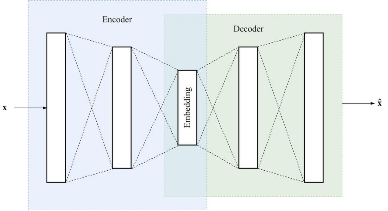
Figure 6: Autoencoder.
